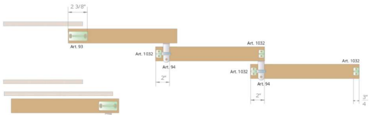
EXAMPLE WITH TWO (2) LEAVES, (For every extra leaf, add two (2) art. 1032 and one (1) art. 94)
